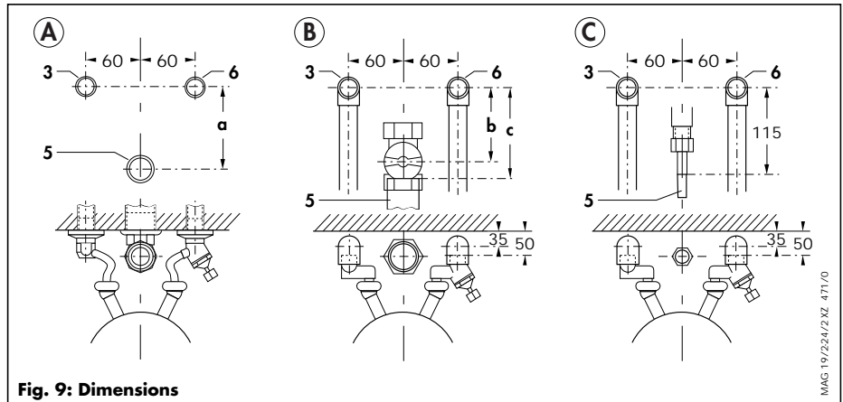
Fig. 9: Dimensions
